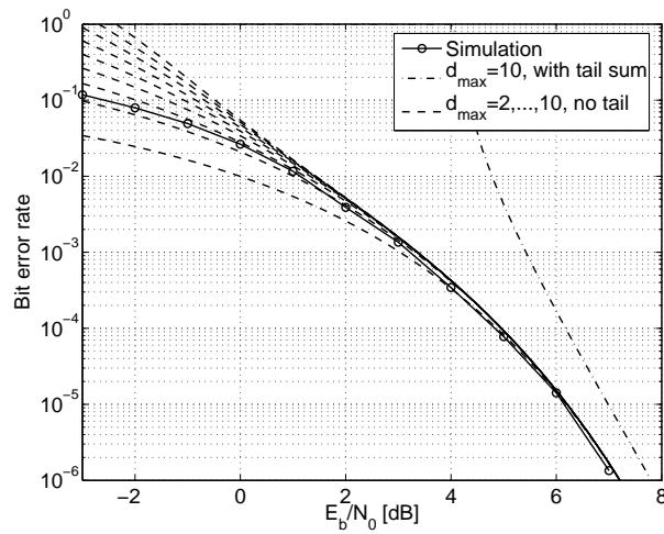
Fig. 3. Approximation of the union bound using matrix inversion: partial sums of (5) up to d = d_{\text{max}} , where d_{\text{max}} = 2, 3, \dots, 10 ; proper upper bound including tail sum (33) with d_{\text{max}} = 10 , \kappa_{\infty} = 2.6 .
