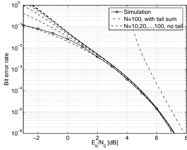
Fig. 2. Recursive approximation of the union bound: partial sum of (5) up to d = 10 , using partial sums of (10) up to n = N , where N = 10, 20, \dots, 100 (evaluated with (11)); proper upper bound including bounded error terms (30) and tail sum (33) with d_{\text{max}} = 10 , N = 100 , \kappa_{\infty} = 2.6 .
