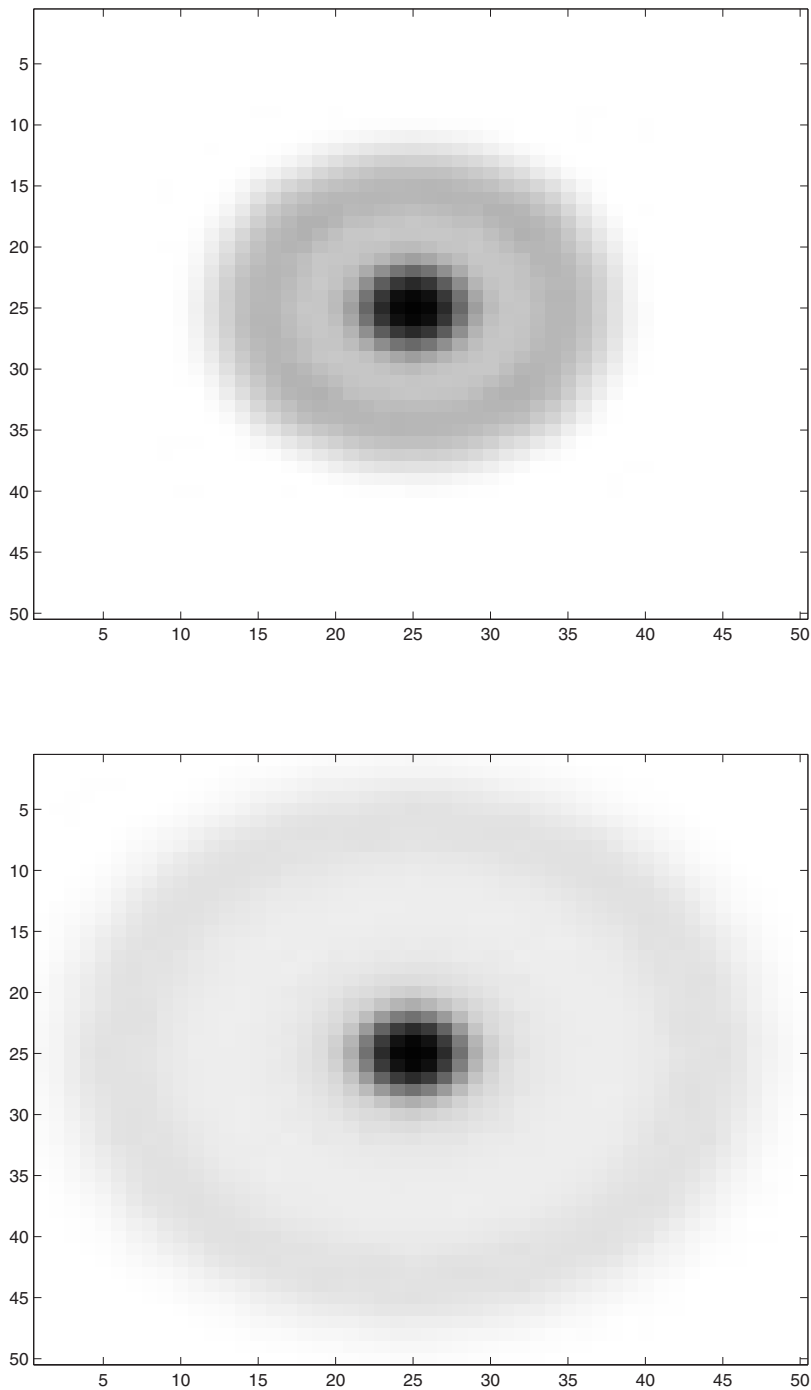
FIGURE 4 Series of secondary images parameterized by scattering angles ( \theta = 36^\circ , 53^\circ and 90^\circ respectively).
